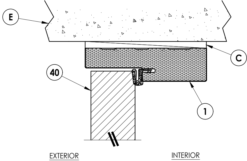
3 5 VERTICAL CROSS SECTION Shown Direct to Masonry Outswing Shown (Inswing Similar)
